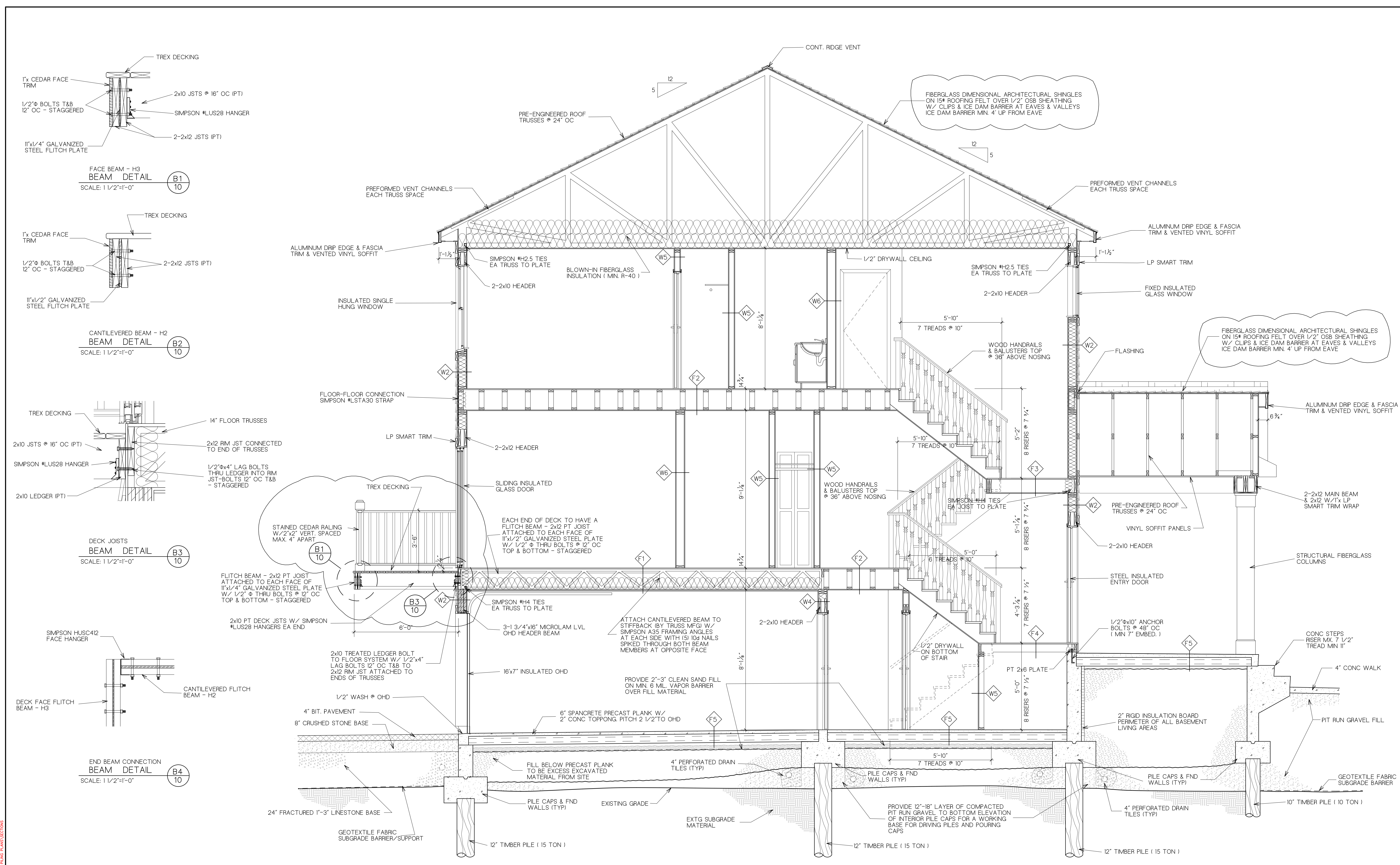
BUILDING SECTION 1 SCALE: 1/2"=1'-0"
